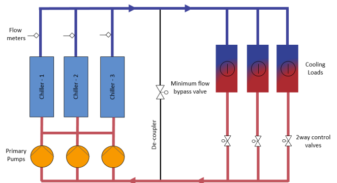
Variable primary flow system
