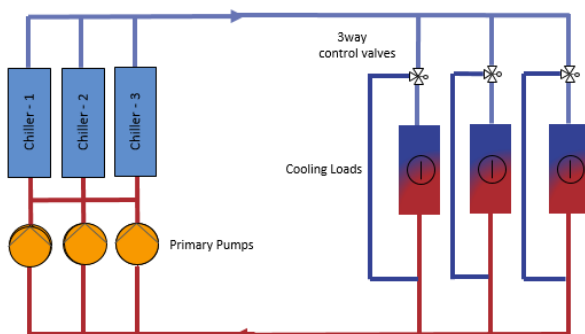
Constant flow primary pumping system
