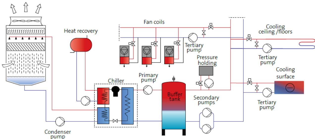
Schematic of a primary / secondary / tertiary chilled water system
