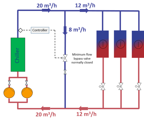
Variable primary flow system with bypass valve
