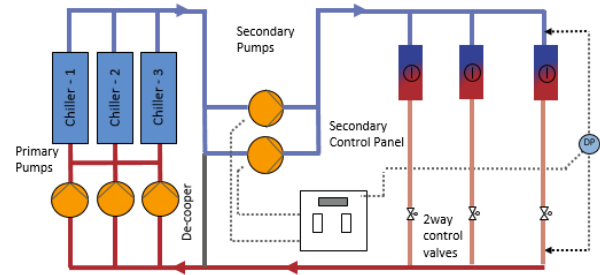
Primary-secondary pumping system
