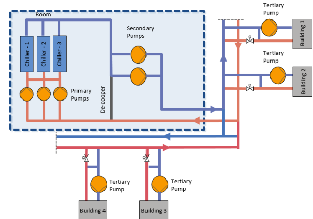
Primary-secondary-tertiary pumping system
