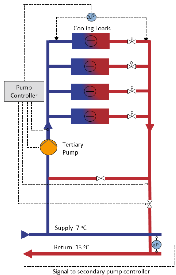
Tertiary pumping system
