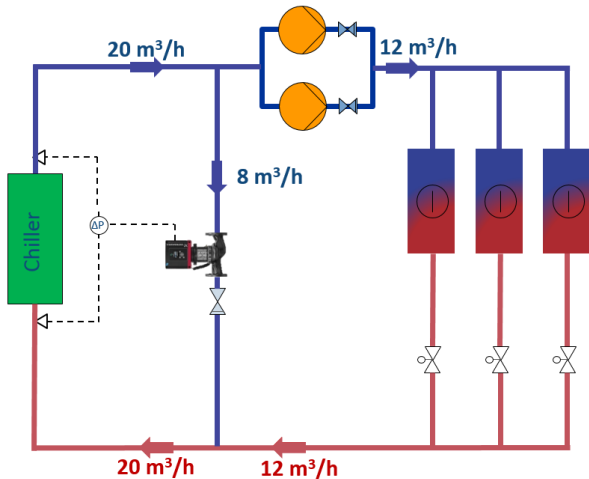
Variable primary flow system with bypass pump
